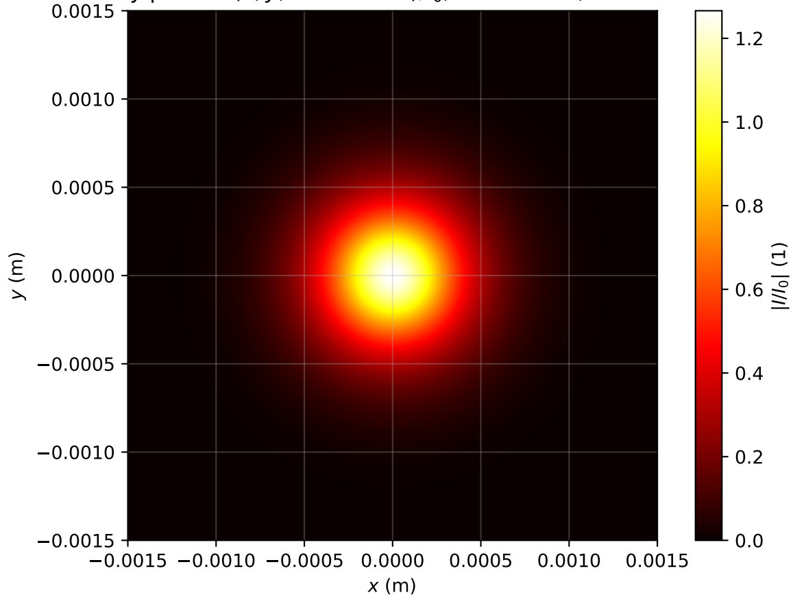
Intensity profile I(x, y, z = 0.637m)/I_0 , Pin=1.0Pcr, artificial time
